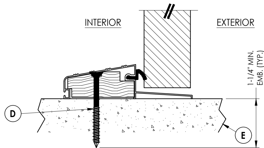
3 3 VERTICAL CROSS SECTION Outswing Sill
