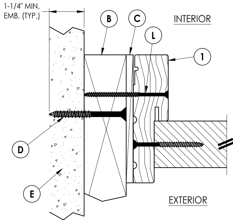
4 HORIZONTAL CROSS SECTION 2 Outswing 1X Buck Construction
